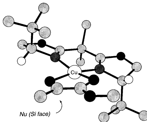
FIGURE 8. PM3-calculated structure of [Cu( S,S )- t -Bu-box](pyruvate)] 2+ .
